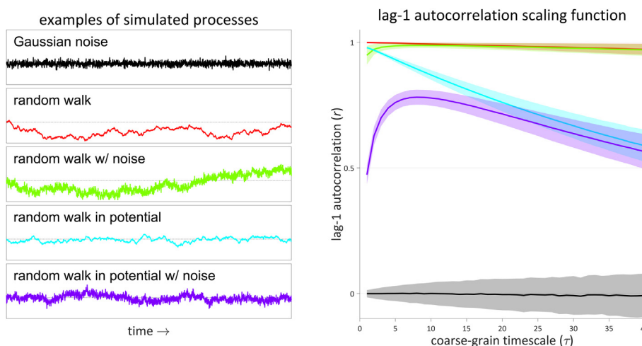
Fig. 1. Comparison of autocorrelation scaling functions of several random processes. (Left) example time series. (Right) Lag-1 autocorrelation scaling functions. Filled areas are \pm 1 s.d. of autocorrelation functions from 1000 simulations of 5000-sample observation sequences.
